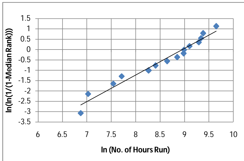
Fig.2 Fitting a line to the data of Type-II
