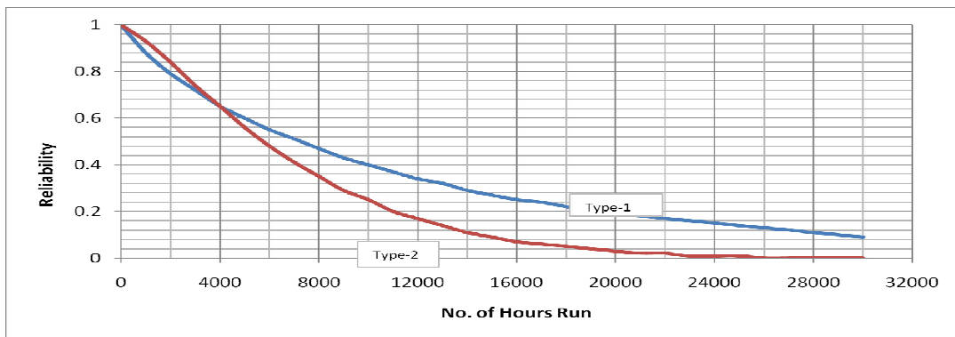
Fig. 5 Graph showing the reliability comparisons of Bulldozers
