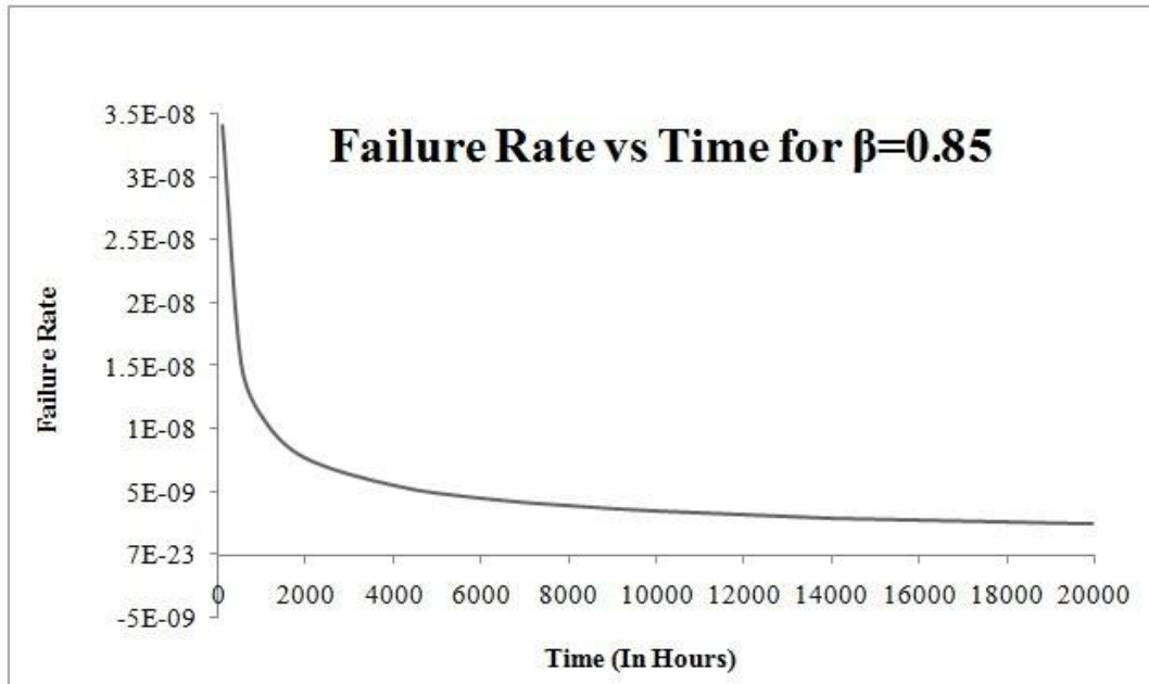
Fig. 3 Graph for Failure Rate vs Time for Type-I Bulldozer(Infant Mortality Rate)
