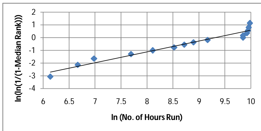
Fig.1 Fitting a line to the data of Type-I
