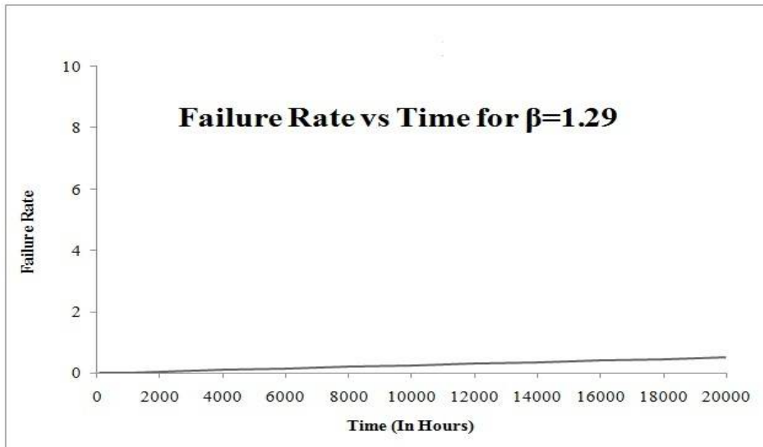
Fig. 4 Graph for Failure rate vs Time for Type-II
